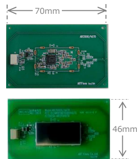
ARI3000X/4670外観
